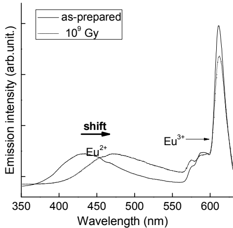
Fig.1. Emission spectra, measured at room temperature, of as-prepared and irradiated ABS glasses containing 3wt% of \text{Eu}_2\text{O}_3 . Excitation with fourth harmonic of Nd:YAG laser (266nm)
