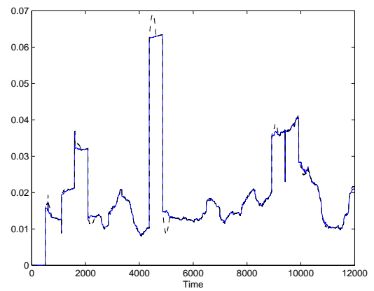
(e) \text{vol}(IBM)(t) (-) and 20 days forecasting (- -)
