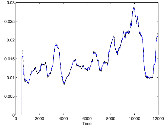
(b) \text{vol}(\text{IBM})(t) (—) and 20 days forecasting (---)
