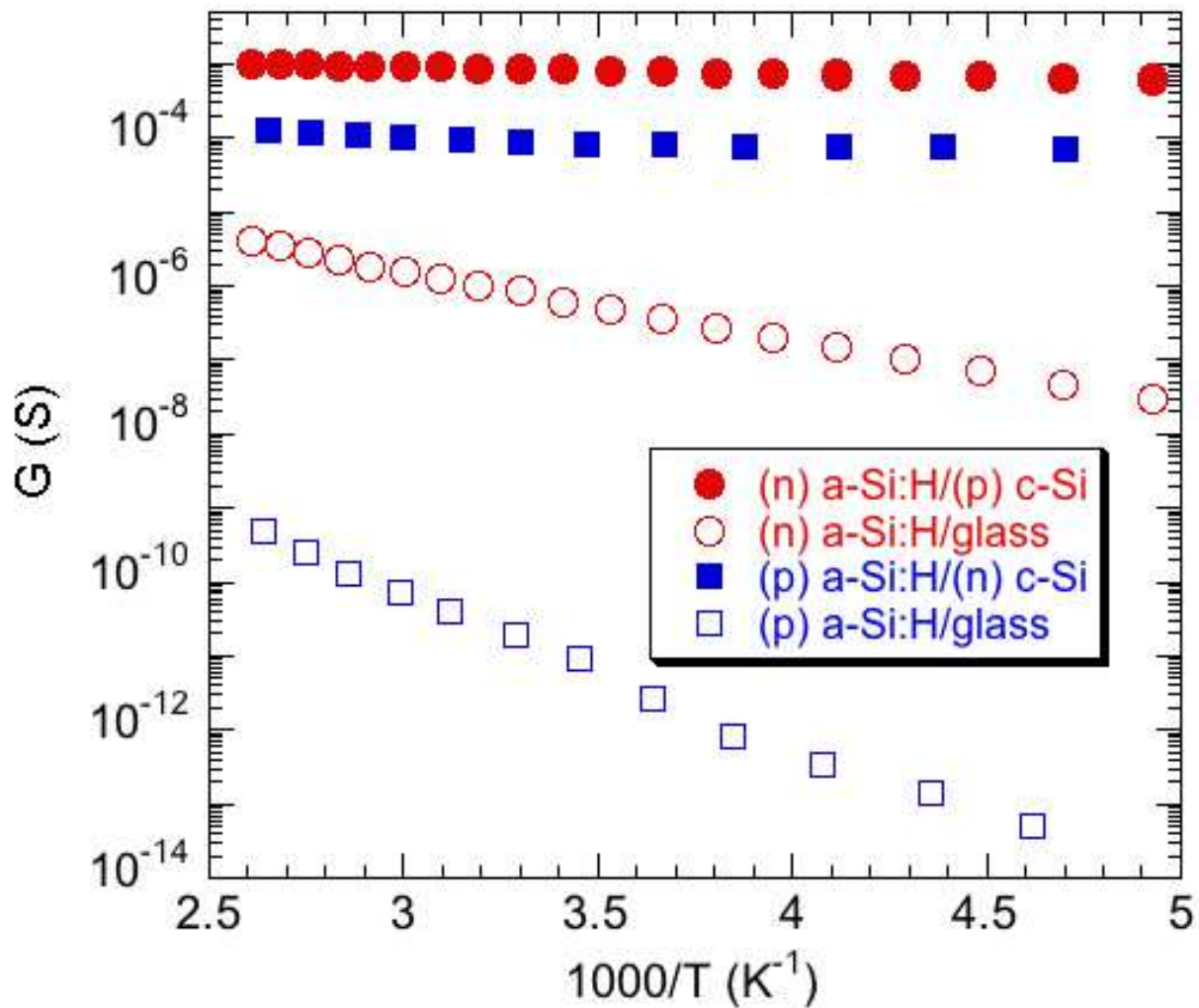
Figure 7 Arrhenius plots of the planar conductance measured on various samples. Red circles for (n) a-Si:H, blue squares for (p) a-Si:H, full symbols for layers deposited on c-Si wafer (on opposite doping type with respect to the deposited a-Si:H layer), open symbols for layers deposited on glass.
