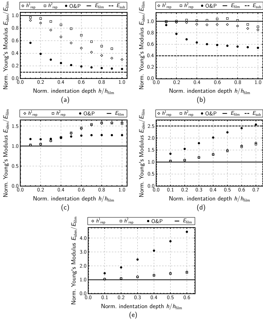
Fig. 5 Identified Young's modulus for the flat punch model using h_{rep} = h_{rep}^1 and h_{rep}^2 , and contact areas evaluated from the Oliver and Pharr method. A comparison is given with estimated values from the Oliver and Pharr method denoted here by O&P. The results are presented for the following film - substrate combinations: (a) E_{film}/E_{sub} = 10 , (b) E_{film}/E_{sub} = 5/2 , (c) E_{film}/E_{sub} = 1 , (d) E_{film}/E_{sub} = 2/5 and (e) E_{film}/E_{sub} = 1/10
