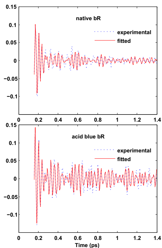
FIGURE 3 Vibrational part of the interferogram of the native sample fitted with seven vibrational modes, and the acid blue sample fitted with nine modes.
