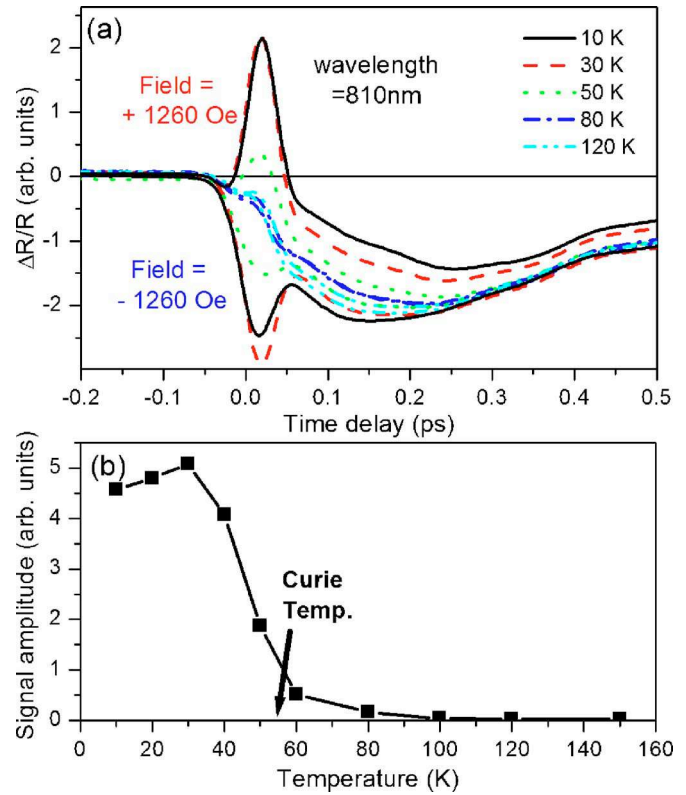
FIG. 3. (Color online) (a) Transient reflection changes at different sample temperatures observed at +1260 and -1260 G, at center wavelength 810 nm, and polarization configuration (C^+, C^+) . (b) Amplitude of coherent artifact signal as a function of applied sample temperature. The amplitude value was obtained by subtracting the signal at -1260 G from that at +1260 G.
