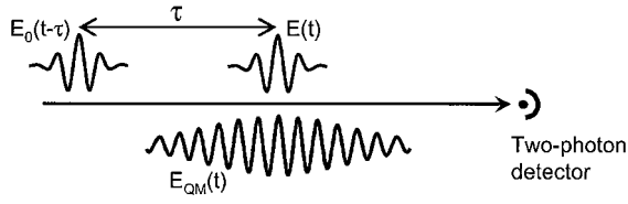
Fig. 2. Time-domain HOT SPIDER. The second-order nonlinear signal is recorded by a two-photon time-integrating detector as a function of time delay \tau between a reference pulse, E_0 , and a superposition of two pulses: the pulse to be measured, E , and a quasi-monochromatic pulse, E_{QM} .
