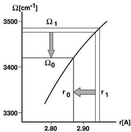
FIG. 1. Relation between the OH \cdots O hydrogen bond length r and the OH link frequency \Omega . r_0 and \Omega_0 designate the equilibrium values of r and \Omega .
