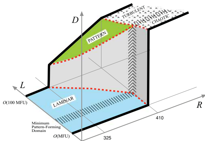
FIG. 2. (Color online) Schematic of the expected bifurcation diagram for PCF including the locations of domains with size of the order of the MFU, and that of pattern-forming systems.
