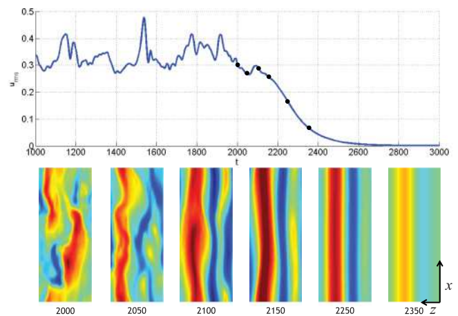
FIG. 6. (Color online) Top: Distance to laminar flow ( U_{\text{rms}} ) during the end of the transient at R = 380 for L = 16.9 . Bottom: Snapshots during decay; time, corresponding to points on the graph, is indicated below the images; exceptionally, the streamwise direction is along the vertical.
