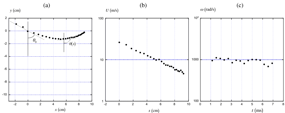
Figure 4. (a) Trajectory of a ball (radius R = 3.5 \text{ mm} , density \rho_s = 920 \text{ kg m}^{-3} ) impacting water with a velocity U_0 = 27 \text{ m s}^{-1} , a spin \omega_0 = 1000 \text{ rad s}^{-1} and an inclination angle \theta_0 = 70^\circ . The time step between two data points is \Delta t = 384 \mu\text{s} . (b) Evolution of the corresponding velocity as a function of the curvilinear location s in a semi-log plot. (c) Time variation of the corresponding rotation speed \omega of the ball.
