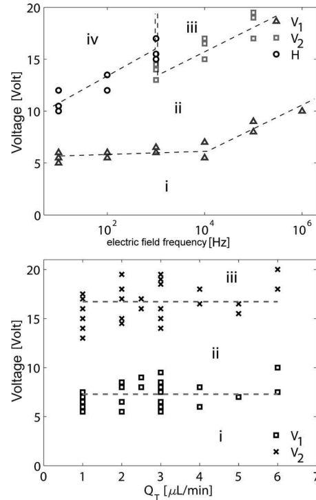
FIG. 6. (Top) Droplet electrocoalescence behavior as a function of the electric field frequency for total flow rates. Q_T = 3 \mu\text{L}/\text{min} and Q_D/Q_T = 0.33 \mu\text{L}/\text{min} ( Q_D = 1 , Q_C = 2 ), 0.5 \mu\text{L}/\text{min} ( Q_D = 1.5 , Q_C = 1.5 ), and 0.66 \mu\text{L}/\text{min} ( Q_D = 2 , Q_C = 1 ). Four regions were identified: (i) no coalescence, (ii) downstream coalescence, (iii) upstream coalescence, and (iv) hydrolysis. (Bottom) Droplet electrocoalescence results from over 30 experiments where Q_T varied from 1 to 6 \mu\text{L}/\text{min} , the ratio Q_D/Q_T varied from 0.28 up to 0.7 and the frequency was fixed at 10 kHz. Dashed lines indicate mean values. The following values were calculated for a distance between electrodes of 20 \mu\text{m} (inset E_2 in Fig. 1): obtaining a mean value of 7.24 V for V_1 and 16.1 V for V_2 , which convert in electric field strength values of 3.62 and 8.05 kV/cm, respectively. At 10 kHz hydrolysis never occurred and region of type (i)–(iii) were obtained.
