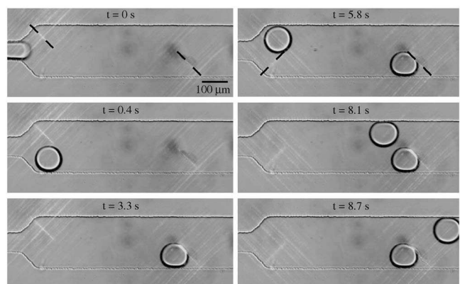
FIG. 3. Image sequence (left column followed by right column) showing how the drop order can be changed: The initial drop is sent down and held stationary, then successive droplets are sent up. The dashed lines overlay the position of the laser patterns.
