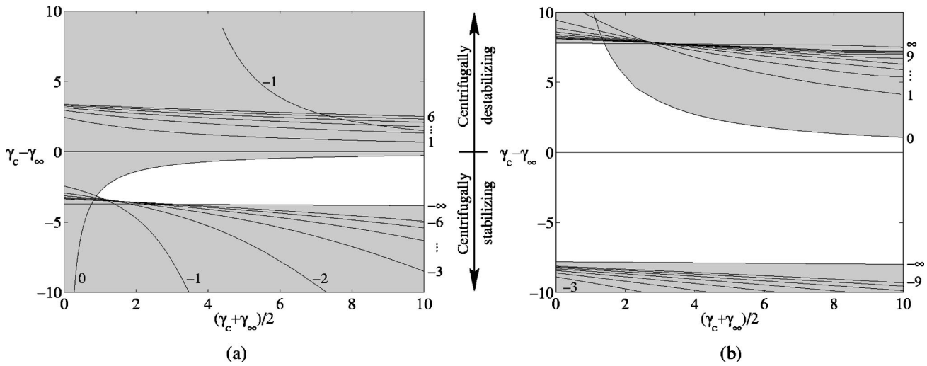
FIG. 3. AI/CI domains in the (\gamma_c + \gamma_\infty)/2 - (\gamma_c - \gamma_\infty) plane for (a) an external counterflow jet at a = -0.2 and (b) an external co-flow jet at a = 0.1 . The shaded area corresponds to the absolutely unstable region, and the clear area to the convectively unstable region. The line \gamma_c - \gamma_\infty = 0 separates the centrifugally stabilizing region ( \gamma_c - \gamma_\infty < 0 ) and the centrifugally destabilizing region ( \gamma_c - \gamma_\infty > 0 ).
