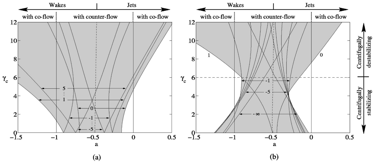
FIG. 4. AI/CI domains in the a - \gamma_c plane for (a) a zero-external swirl ( \gamma_\infty = 0 ) and (b) a finite external swirl ( \gamma_\infty = 6 ). The shaded area corresponds to the absolutely unstable region, and the clear area to the convectively unstable region. The dotted line \gamma_c = \gamma_\infty separates the centrifugally stabilizing and destabilizing regions. For clarity, in (b), only the helical modes participating in the delineation of the AI/CI regions have been represented.
