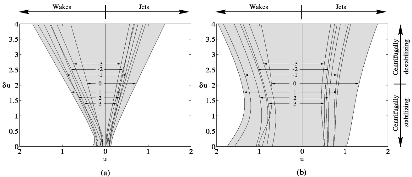
FIG. 5. AI/CI domains in the \bar{u} - \delta u plane for (a) \delta\gamma=1.5 and (b) \delta\gamma=0.01 . The shaded area corresponds to the absolute unstable region, and the clear area to the convectively unstable region.
