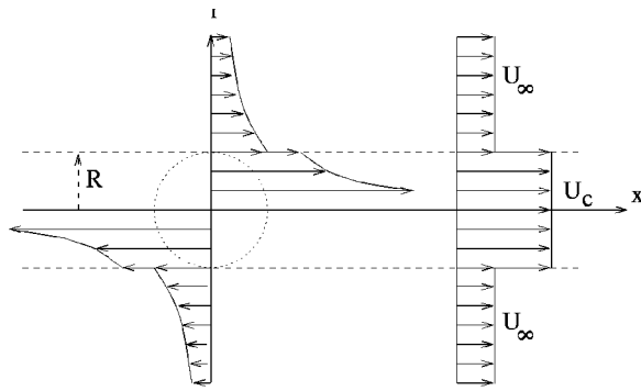
FIG. 1. Sketch of basic flow azimuthal and axial velocity profiles.
