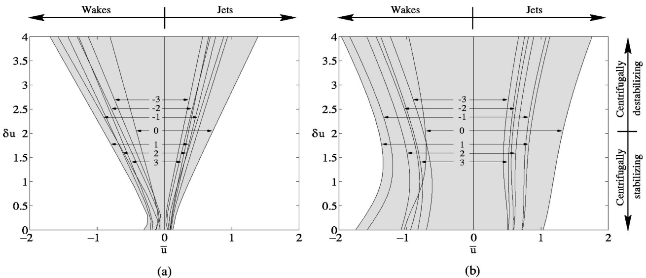
FIG. 5. AI/CI domains in the \bar{u} - \delta u plane for (a) \delta\gamma = 1.5 and (b) \delta\gamma = 0.01 . The shaded area corresponds to the absolute unstable region, and the clear area to the convectively unstable region.
