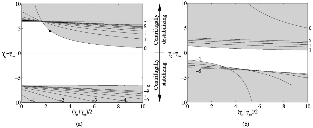
FIG. 2. AI/CI domains in the (\gamma_c + \gamma_\infty)/2 - (\gamma_c - \gamma_\infty) plane for (a) a zero-external axial flow jet ( a=0 ) and (b) a zero-centerline velocity wake ( a=-1 ). The shaded area corresponds to the absolutely unstable region, and the clear area to the convectively unstable region. The line \gamma_c - \gamma_\infty = 0 , separates the centrifugally stabilizing region ( \gamma_c - \gamma_\infty < 0 ) and the centrifugally destabilizing region ( \gamma_c - \gamma_\infty > 0 ). The solid dot in (a) corresponds to the AI/CI transition point \gamma_c = 4.65 , \gamma_\infty = 0 calculated in Ref. 15.
