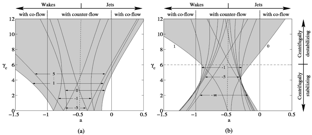
FIG. 4. AI/CI domains in the a - \gamma_c plane for (a) a zero-external swirl ( \gamma_\infty=0 ) and (b) a finite external swirl ( \gamma_\infty=6 ). The shaded area corresponds to the absolutely unstable region, and the clear area to the convectively unstable region. The dotted line \gamma_c = \gamma_\infty separates the centrifugally stabilizing and destabilizing regions. For clarity, in (b), only the helical modes participating in the delineation of the AI/CI regions have been represented.
