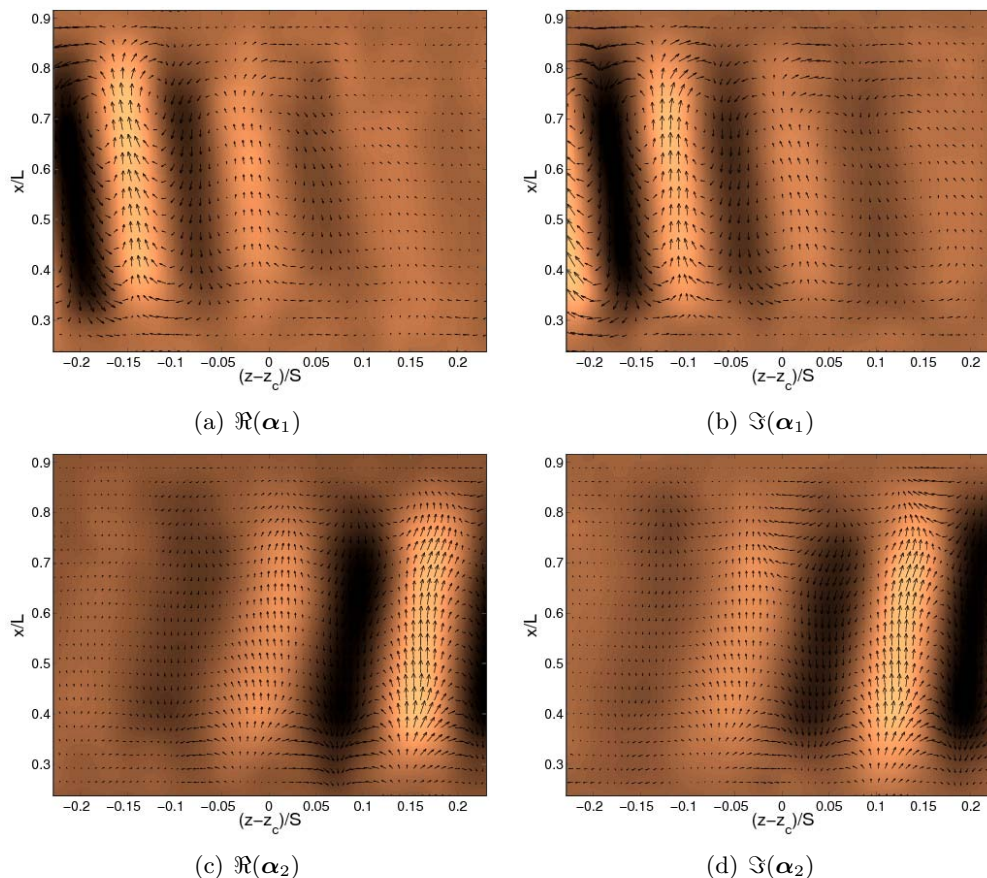
Figure 6. Real and imaginary parts of vectors \alpha_1 and \alpha_2 , associated with f_1 = 0.13 Hz and f_2 = 0.22 Hz. Quivers give the real part ( \alpha_z, \alpha_x ), and color contours represent the real part of \alpha_k \cdot e_x .
