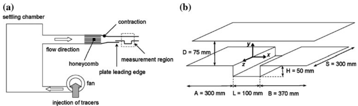
Figure 1. Sketch of the experimental setup, (a) windtunnel, (b) cavity sub-system with L/H = 2 .
