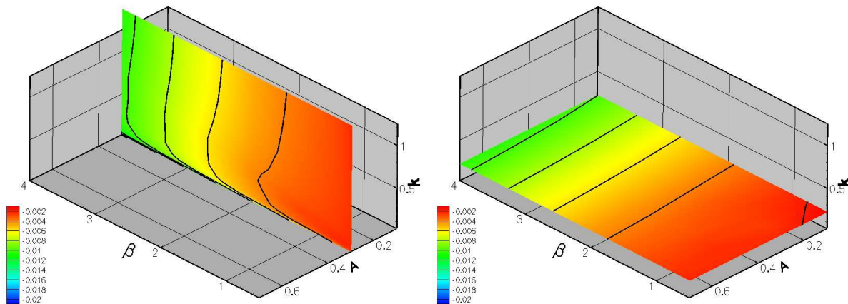
Figure 2. Maximum growth rate at Re = 2000 , as a function of the parameters \kappa , A and \beta .
