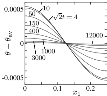
(c) \theta - \theta_{av} ( \sqrt{2}t \leq 12000 )
