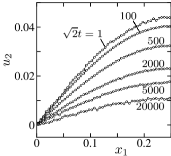
(a) u_2 ( \sqrt{2}t \leq 20000 )
