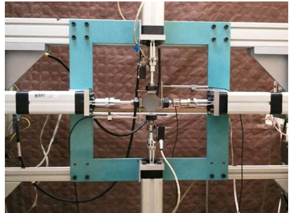
Fig. 4. Biaxial apparatus used for biaxial prestrain DMA experiments with the cruciform shape specimen in the center.
