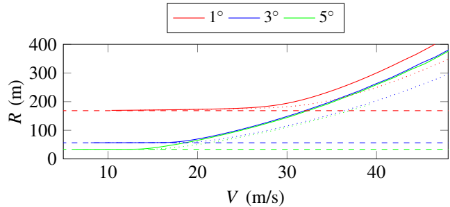
Fig. 11. Radius versus speed for different steering angles obtained with the 9DoF model for \mu = 0.7 (full lines), \mu = 1 (dotted lines) and with the kinematic bicycle model (dashed lines)
