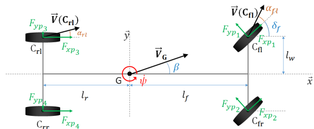
Fig. 3. Simulation model of the vehicle
