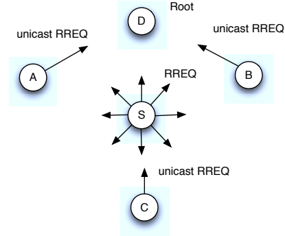
(b) Route discovery with smart route request
