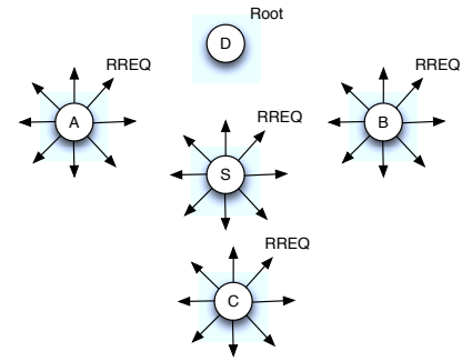
(a) Route discovery without smart route request
