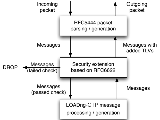
Figure 5: Relationship with RFC5444, RFC6622 and LOADng-CTP
