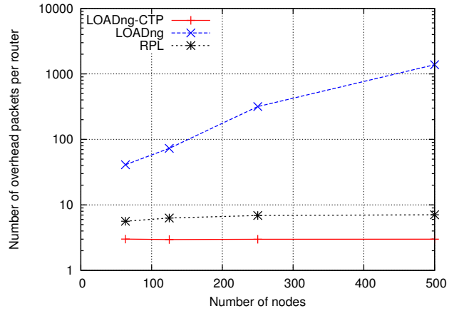
Figure 10: Number of overhead packets transmitted by each router
