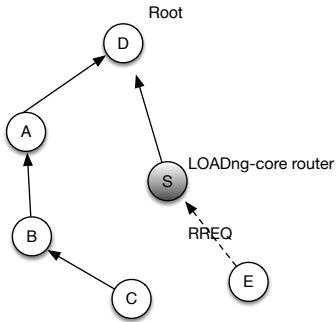
Figure 6: An example of interoperability between LOADng-CTP (white nodes) and LOADng-core routers (grey nodes).
