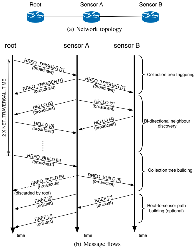
Figure 2: Message exchange of LOADng-CTP between root and sensors
