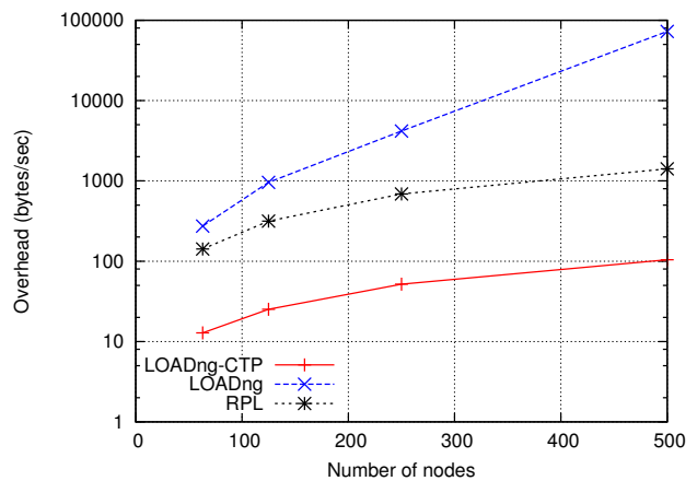
Figure 11: Overhead bytes per second in the whole network
