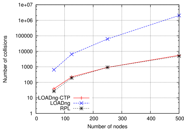
Figure 8: Number of MAC layer collisions
