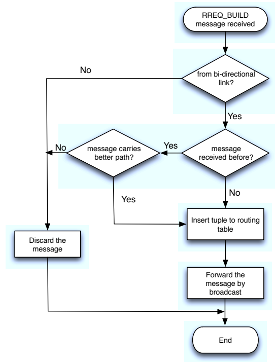
Figure 1: LOADng-CTP RREQ_BUILD message processing
