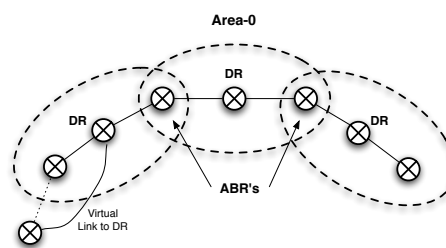
Fig. 1. An OSPF autonomous system splitted in different areas (Area-0 is the backbone area).
