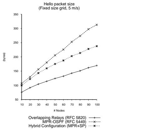
Fig. 12. Average size of Hello packets (fixed grid, 5 m/s).
