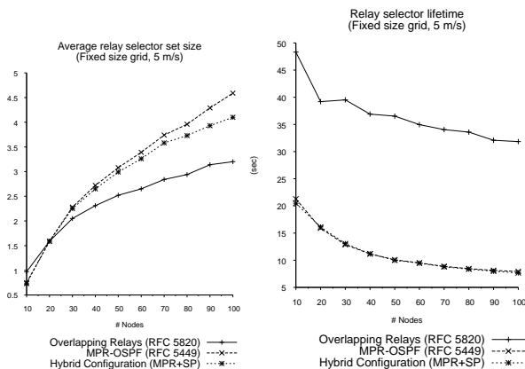
Fig. 10. (a) Average number of relays per node and (b) average relay lifetime (fixed size grid, 5 m/s).
