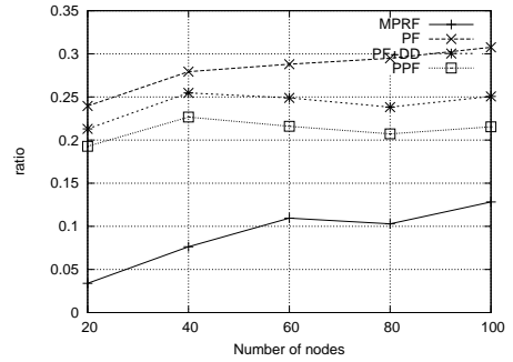
Figure 5. Collision ratio
