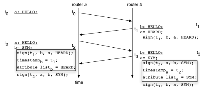
Fig. 2. Example of link admittance control in the Neighborhood Discovery process of OLSRv2: attributes listed in “boxes” are those received from the “peer” in a previous HELLO message.
