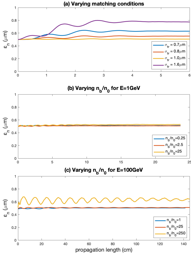
FIG. 3. Evolution of the normalized transverse emittance of the trailing positron bunch, \varepsilon_n = \sqrt{\langle x^2 \rangle \langle p_x^2 \rangle - \langle x p_x \rangle^2} / mc , during its propagation in the plasma. For all simulations, the plasma density is set to n_0 = 5 \times 10^{16} \text{ cm}^{-3} , the peak density of the electron drive bunch is n_b = 0.35 n_0 , the drive beam size and bunch length are \sigma_{dr} = 14.5 \mu\text{m} and \sigma_{dz} = 16.7 \mu\text{m} , the drive beam evolution is turned off, and the drive to trailing bunch separation is \Delta\xi = 143 \mu\text{m} . The initial trailing positron bunch energy is 1 GeV in (a) and (b) and 100 GeV in (c). The matching condition is varied in (a), while the trailing positron beam is quasimatched for increasing values of n_b/n_0 in (b) and (c). All initial trailing positron beam parameters and corresponding values for efficiency and emittance growth are listed in Table I.
